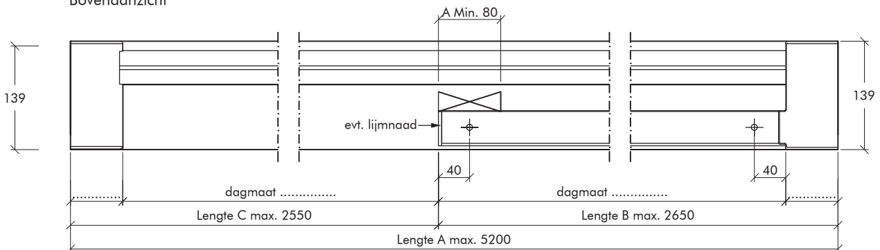
Montage rail Luvema RO.295.G
