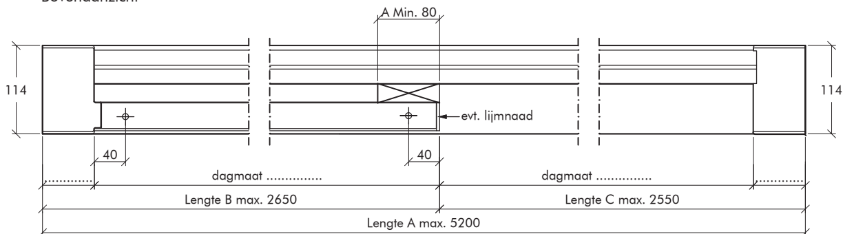
Montage rail Luvema RO.295.G
